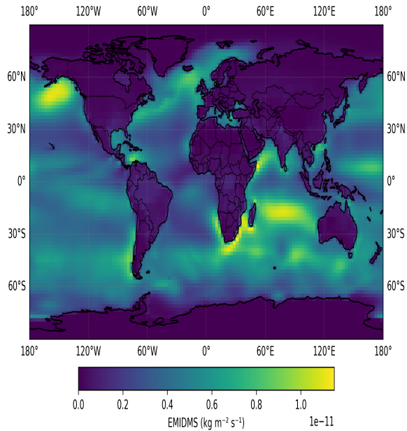
EC-Earth - Global - EMIDMS (baseline)
