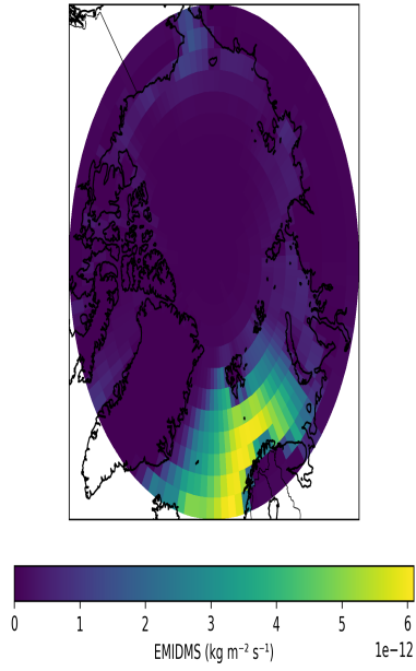
EC-Earth - Arctic - EMIDMS (baseline)
