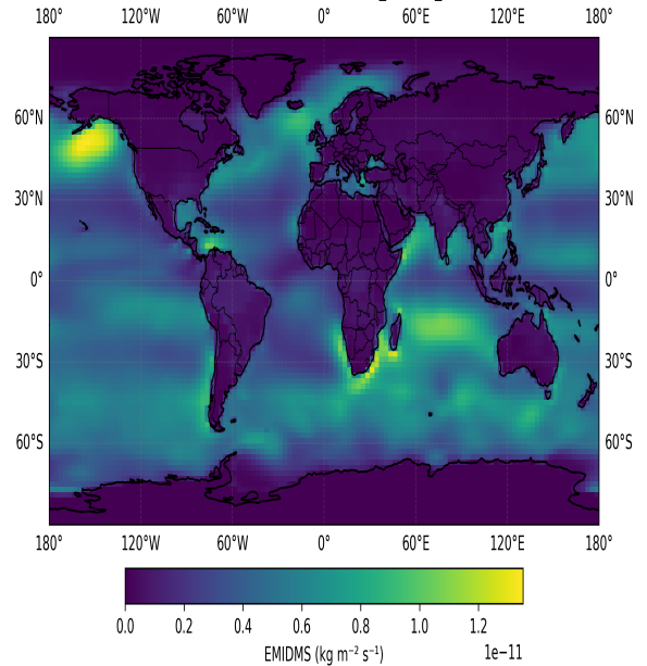
EC-Earth - Global - EMIDMS (SST_contrib_ssp585)
