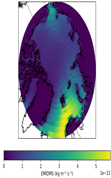
EC-Earth - Arctic - EMIDMS (seaice_contrib_ssp585)
